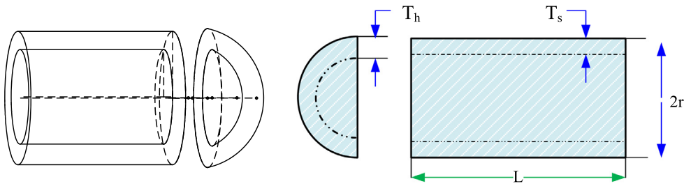
Fig. 14. Pressure vessel problem.
