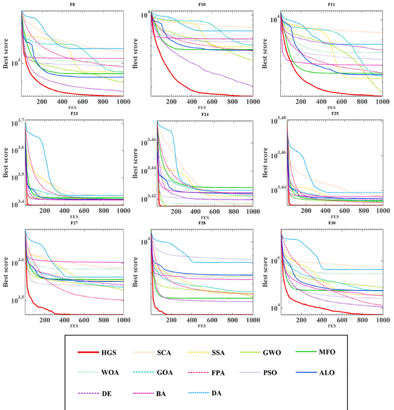
Fig. 7. Comparisons between HGS and traditional MAs.
