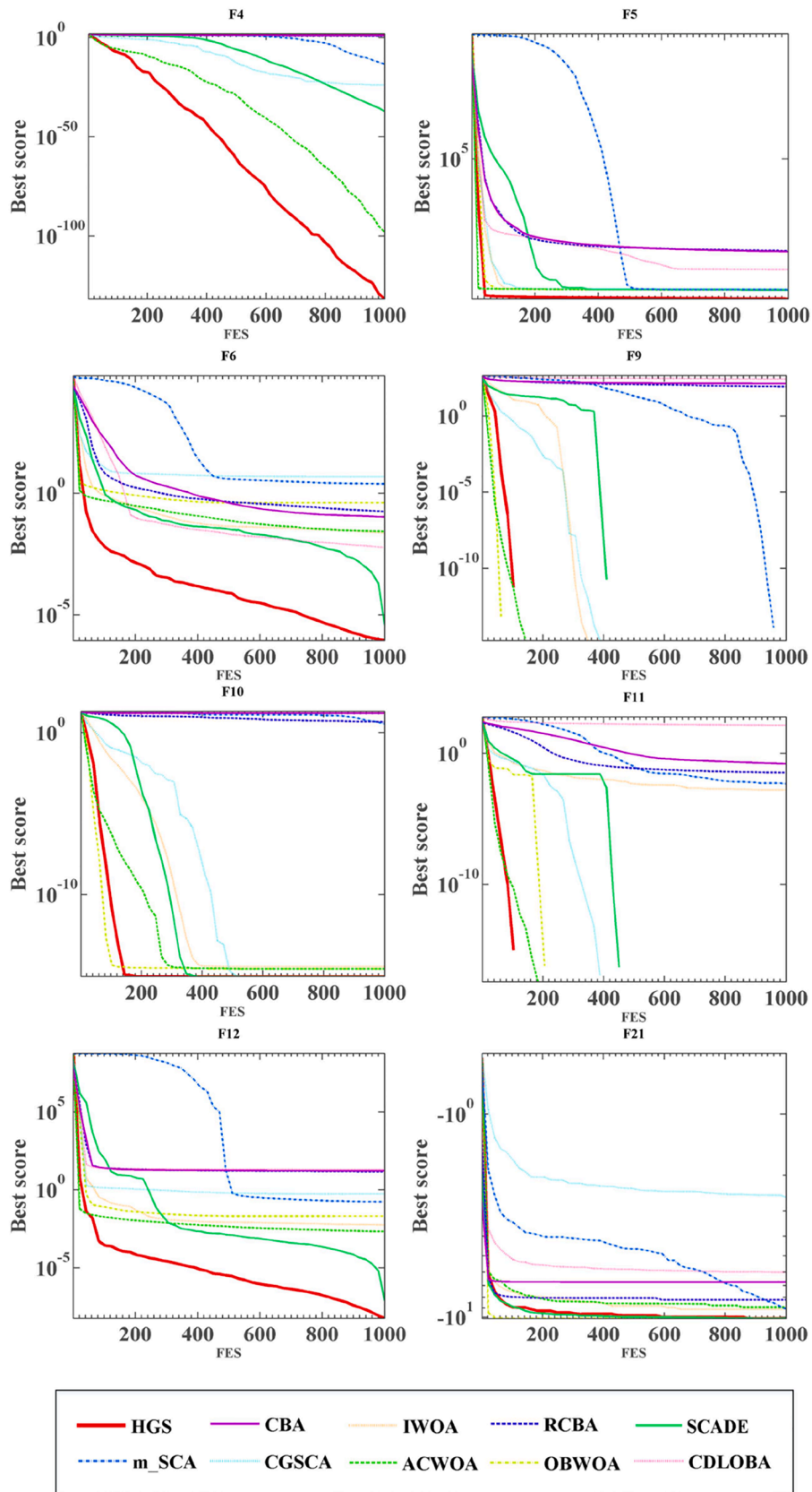
Fig. 6. Comparisons between HGS and advanced MAs.
