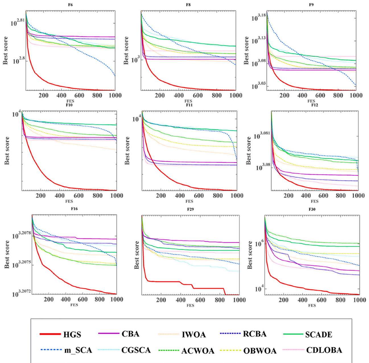
Fig. 8. Comparisons between HGS and advanced MAs.
