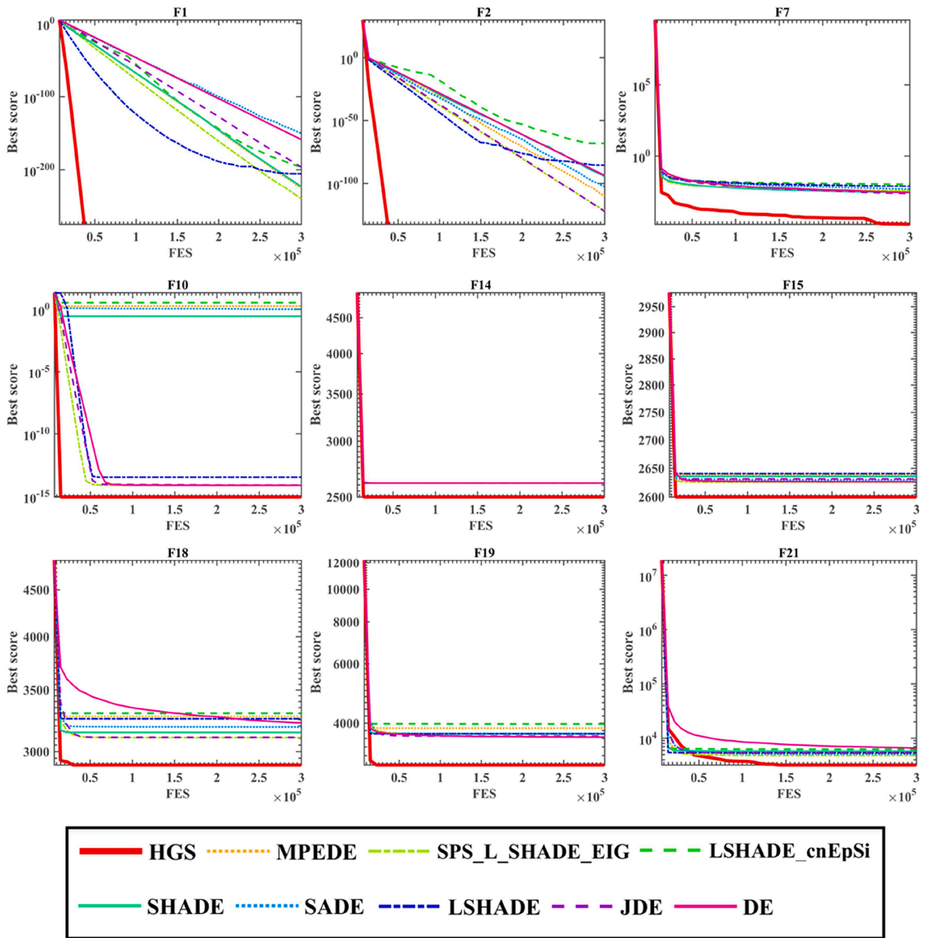
Fig. 9. Comparisons between HGS and DE variants.
