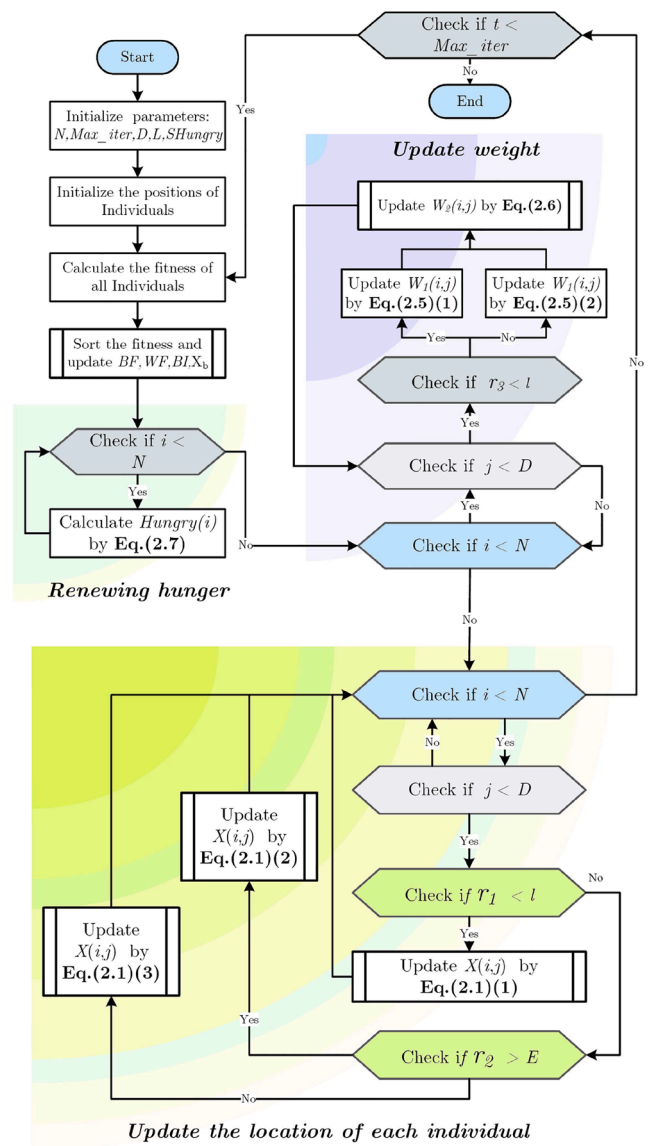
Fig. 3. Flowchart of Hunger Games Search (HGS) algorithm.
