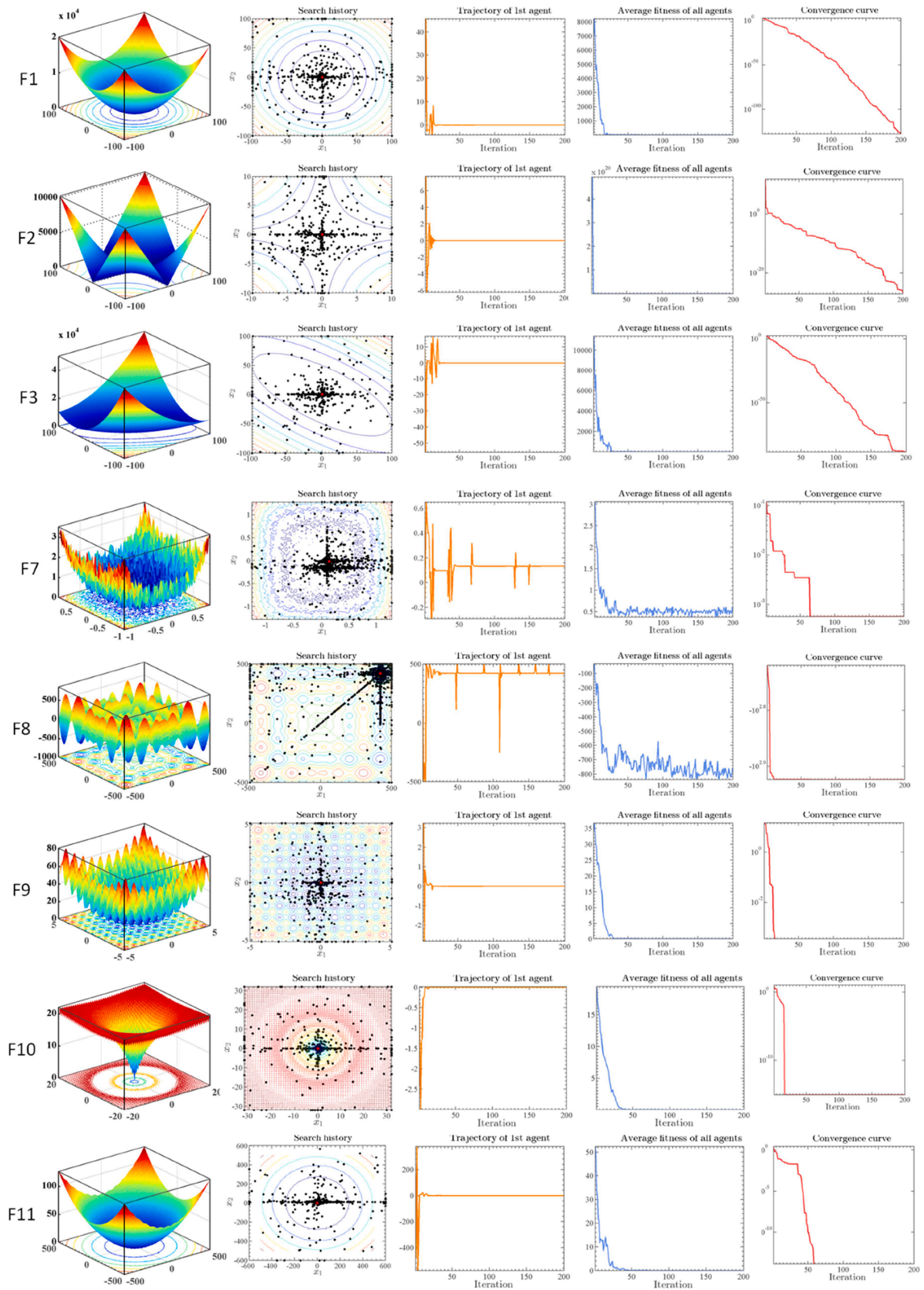
Fig. 4. Qualitative analysis of HGS on some typical functions.
