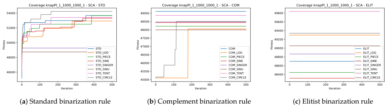
Figure 8. Convergence graphs of the best execution obtained for the knapPI_1_1000_1000_1 instance using SCA.
