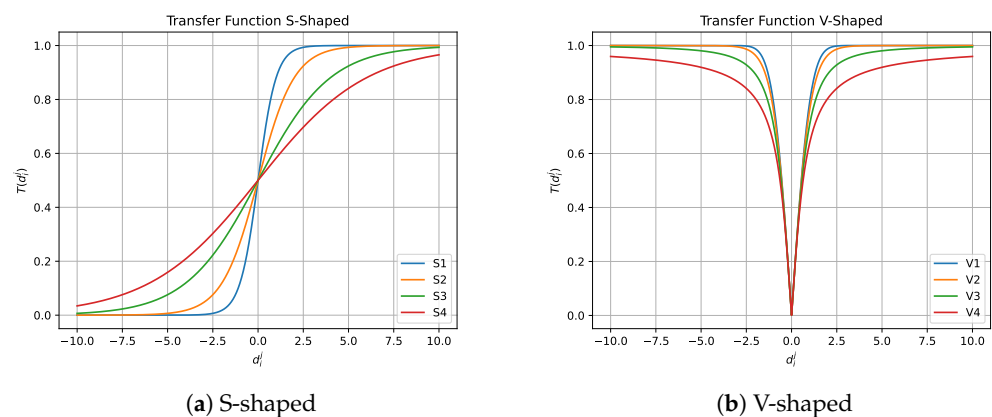
Figure 4. S-Shaped and V-Shaped transfer functions.
