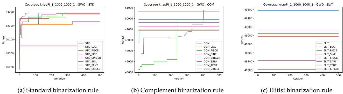
Figure 6. Convergence graphs of the best execution obtained for the knapPI_1_1000_1000_1 instance using GWO.
