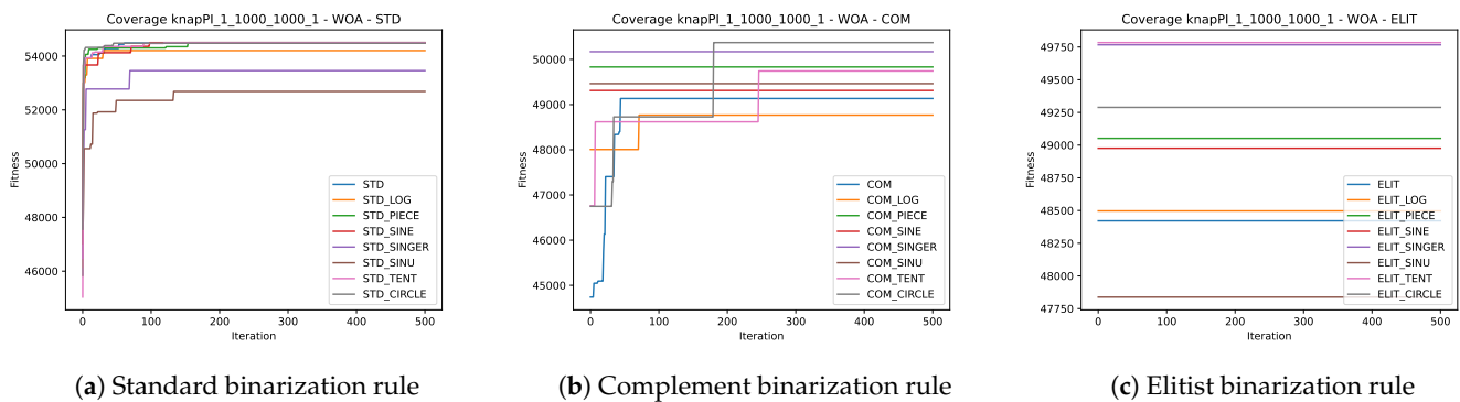
Figure 7. Convergence graphs of the best execution obtained for the knapPI_1_1000_1000_1 instance using WOA.
