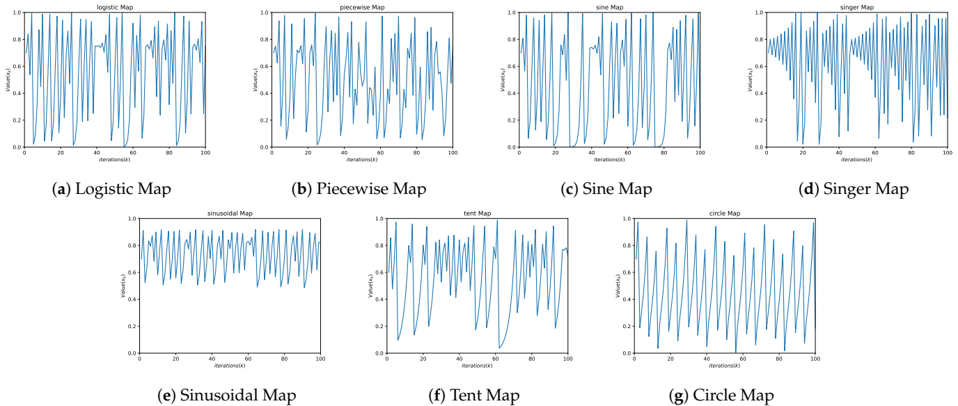
Figure 1. Chaotic maps.
